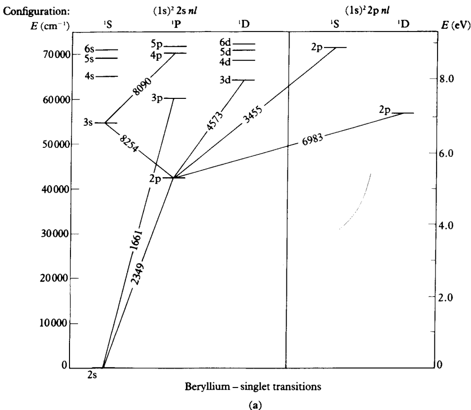
8.5 Grotrian diagram for transitions in beryllium (a) singlet (b) triplet energies are shown relative to the (1s)^2 (2s)^2 \ ^1S ground state. Only a selection of transitions are shown, for sake of clarity. The numbers against the lines show the wavelength in angstroms. The ‘displaced terms’ are shown on the right-hand side of each diagram.
